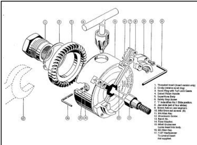
Exploded View of SuperNova Chuck
