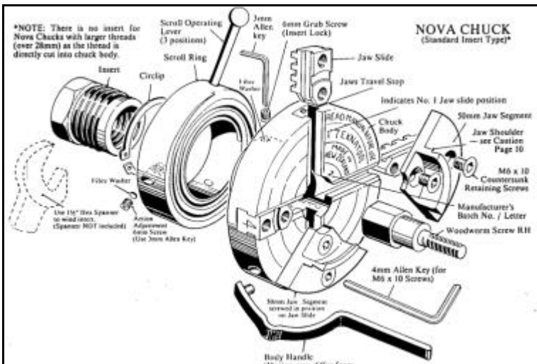
Exploded View of Nova Chuck
